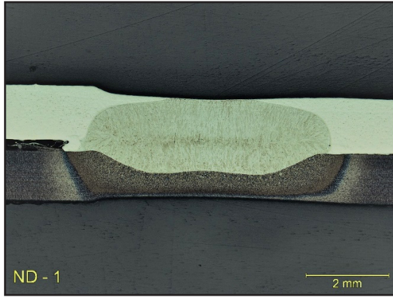
Figure 1. Dissimilar Weld Joint between DP 980 (L/S) and NXG™ 1200 (R/S)
