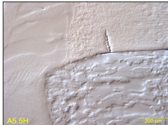
Figure 2. High Magnification of Fusion Boundary in LME Test of NXG™ 1200 Resistance Spot Weld Showing Typical Results in a) and Worst Case b)
